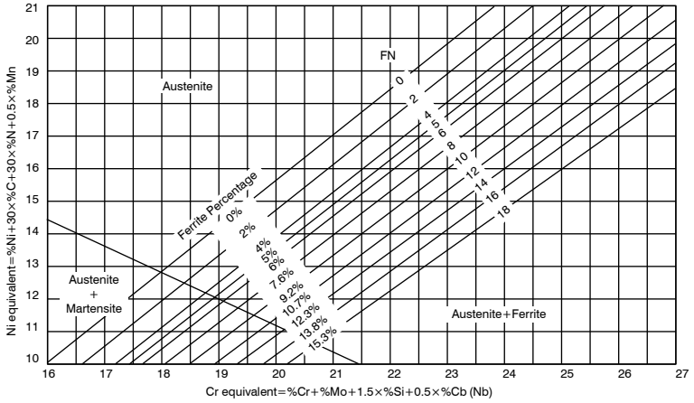
Fig. 2 DeLong Diagram
